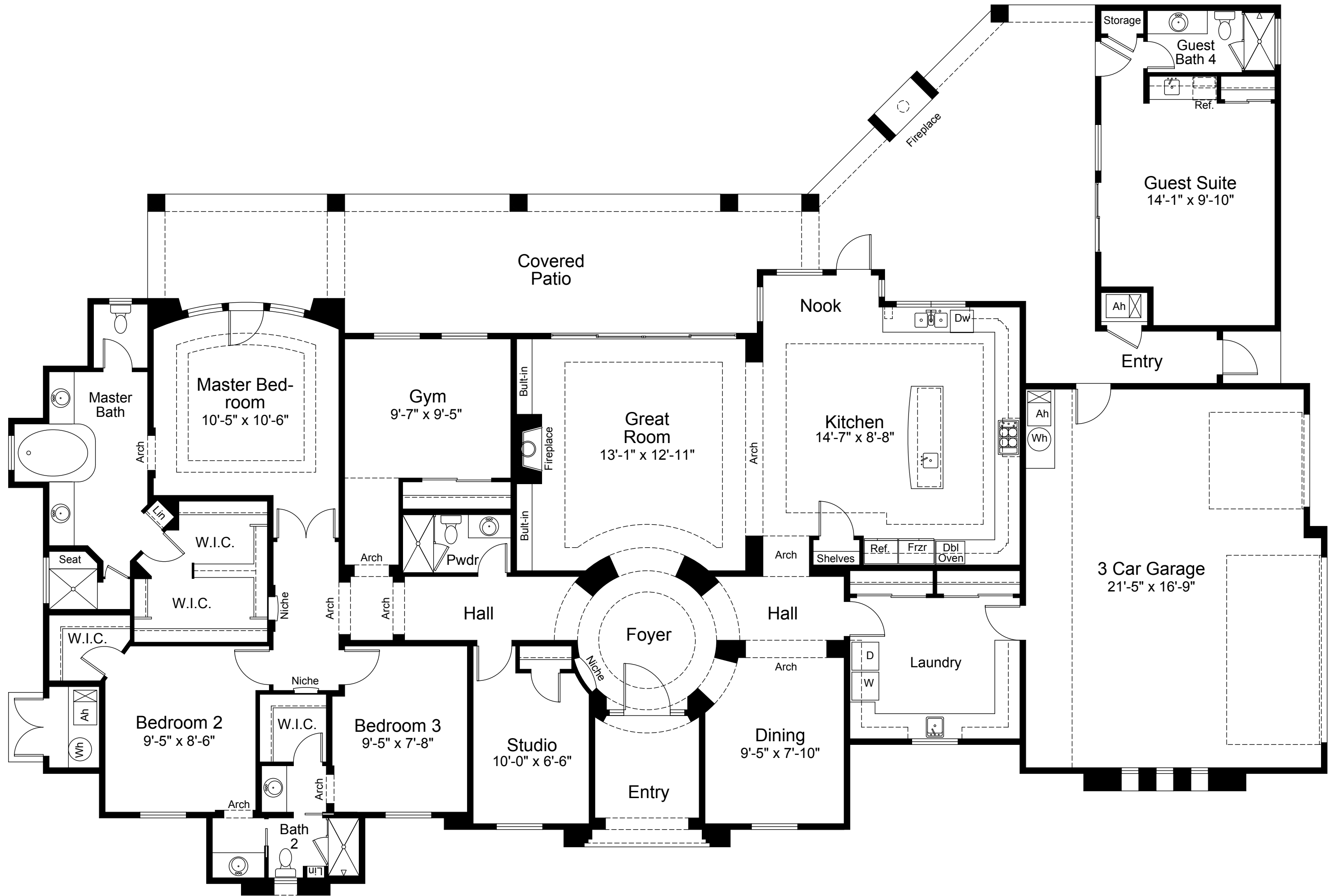
FLOOR PLAN
